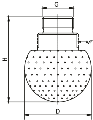
Male Connection
